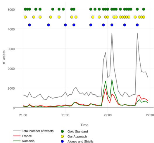
Figure 5: Sub-events in France-Romania.
