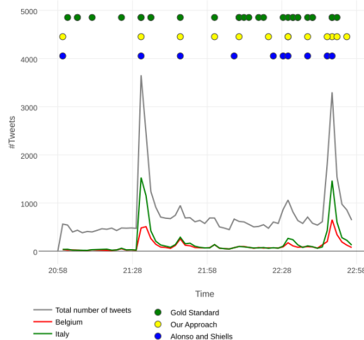
Figure 6: Sub-events in Belgium- Italy.
