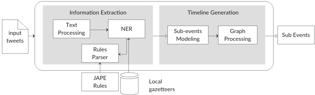
Figure 1: Sub-events extraction pipeline.
