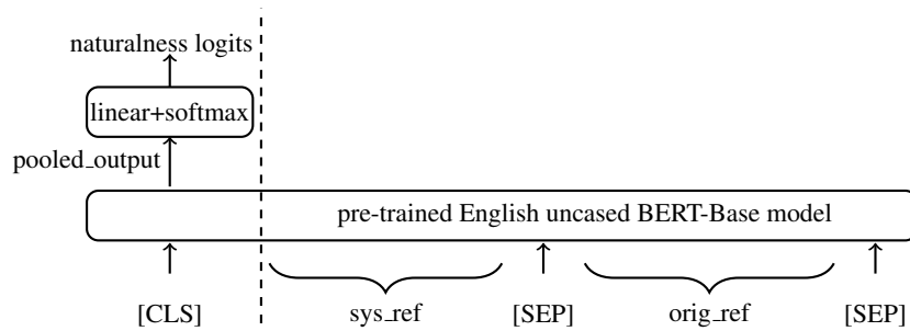
Figure 2: Fine-tuning BERT architecture for naturalness estimation
