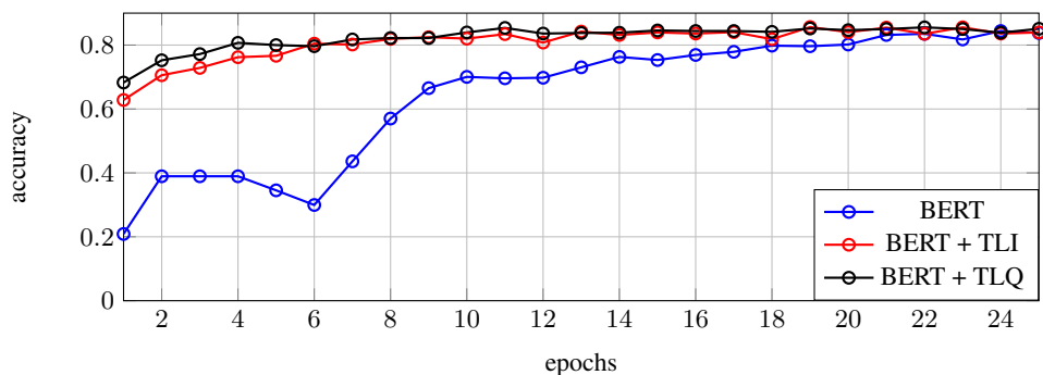
Figure 3: Comparison of the different approaches to naturalness estimation with respect to the training epochs. With additional transfer learning using the quality score (BERT + TLQ), the training speed is increased the most.
